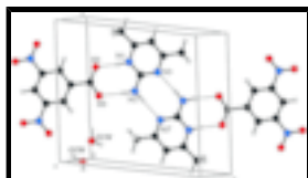
Fig. 2. Hydrogen bonding patterns in the title compound. Symmetry codes: (i) -x, -y + 1, -z + 1 .
