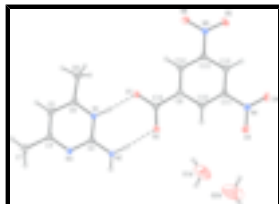
Fig. 1. An ORTEP view of the asymmetric unit of the title compound showing 30% probability displacement ellipsoids. Hydrogen bonds are shown as dashed lines.
